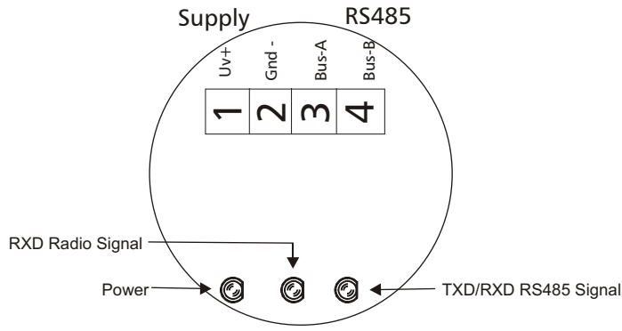
SRC-RS485 Gateway
