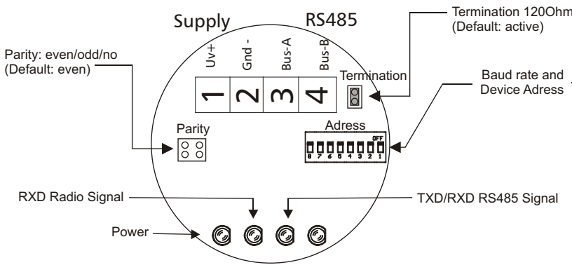
SRC-RS485 EVC
