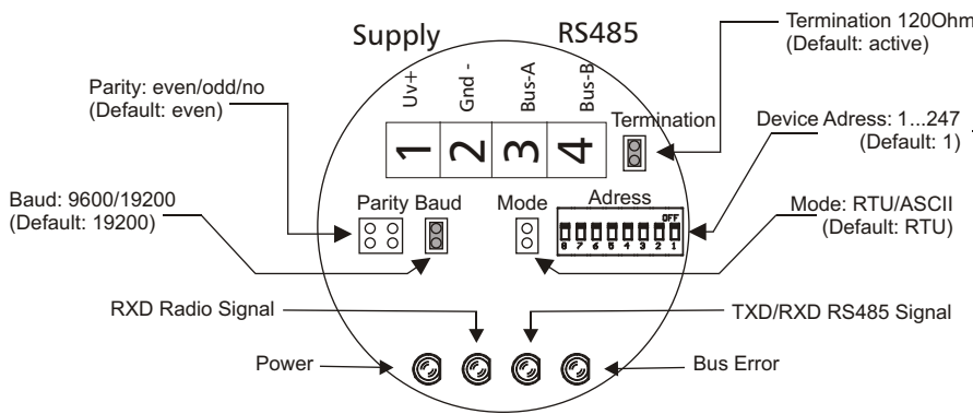
SRC-RS485 Modbus
