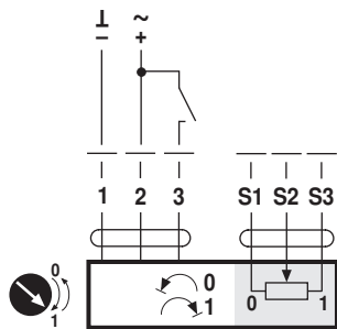
AC/DC 24 V, open-dicht
